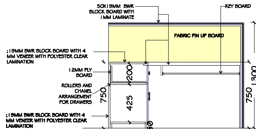
SECTIONAL ELEVATION OF F F'
